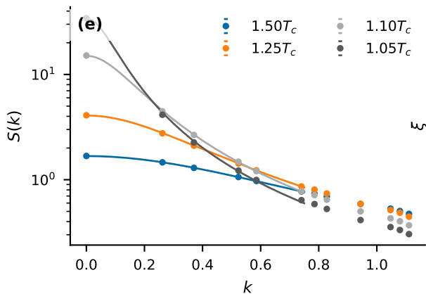
Connected structure factor; fits use k \leq 0.75
