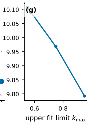
Fit range at 1.05T_c
